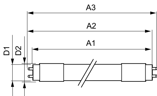
8T5HE/22-850/IF10/G/DIM 10/1
