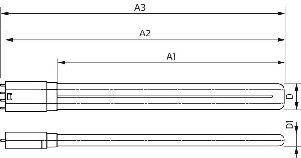
PLL 17W Type B DLC5.1 3500K
