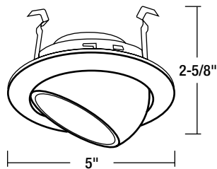
Trim OD: 5" Height: 2-5/8"
