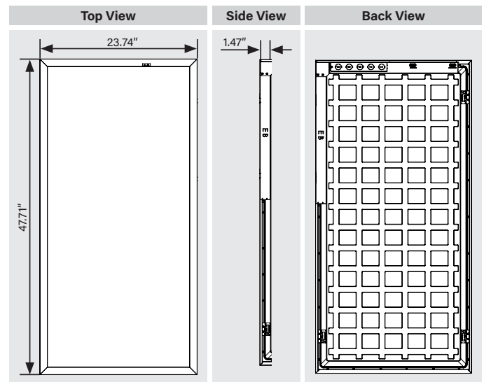
KT-BPLED45PS-24C-8CSA-VDIM-EM8
