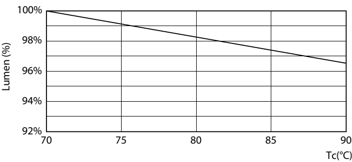
LEDtube_PLCT_11W_30K_LumenVsTc-LMP
