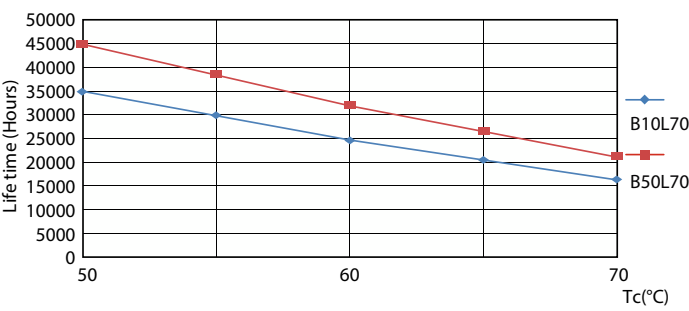
LEDtube_30K_5070_LifetimeVsTc-LED
