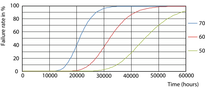
LEDtube_30K_5070_FailureRate-LED
